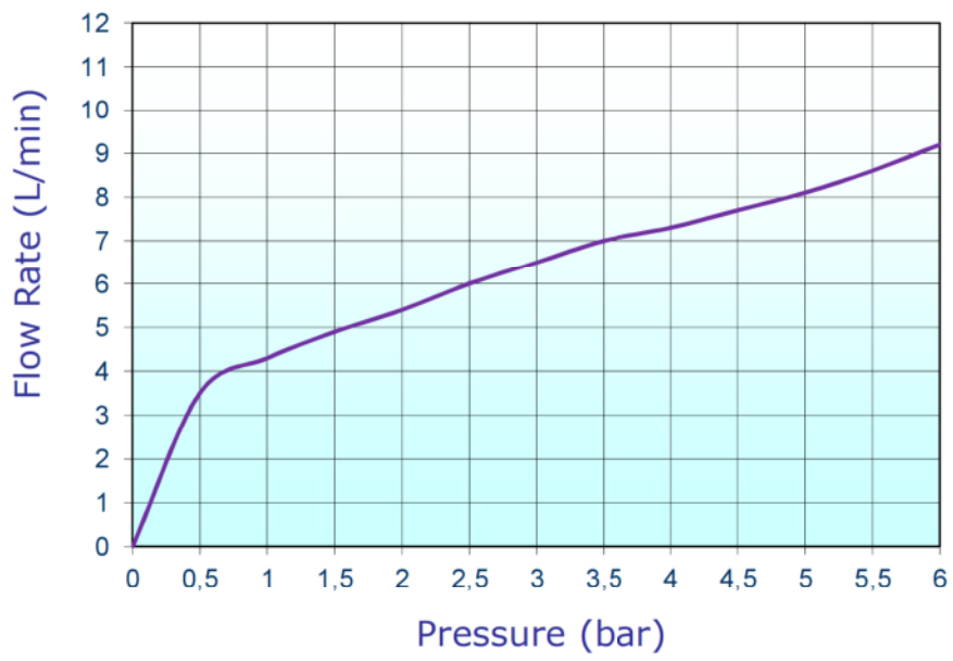
8L565 flow rate
